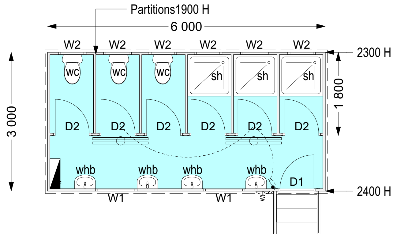
GROUND FLOOR PLAN 1:50
